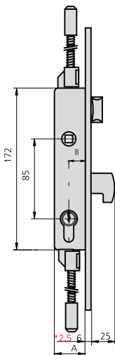
U-SHAPED FRONT PLATE
